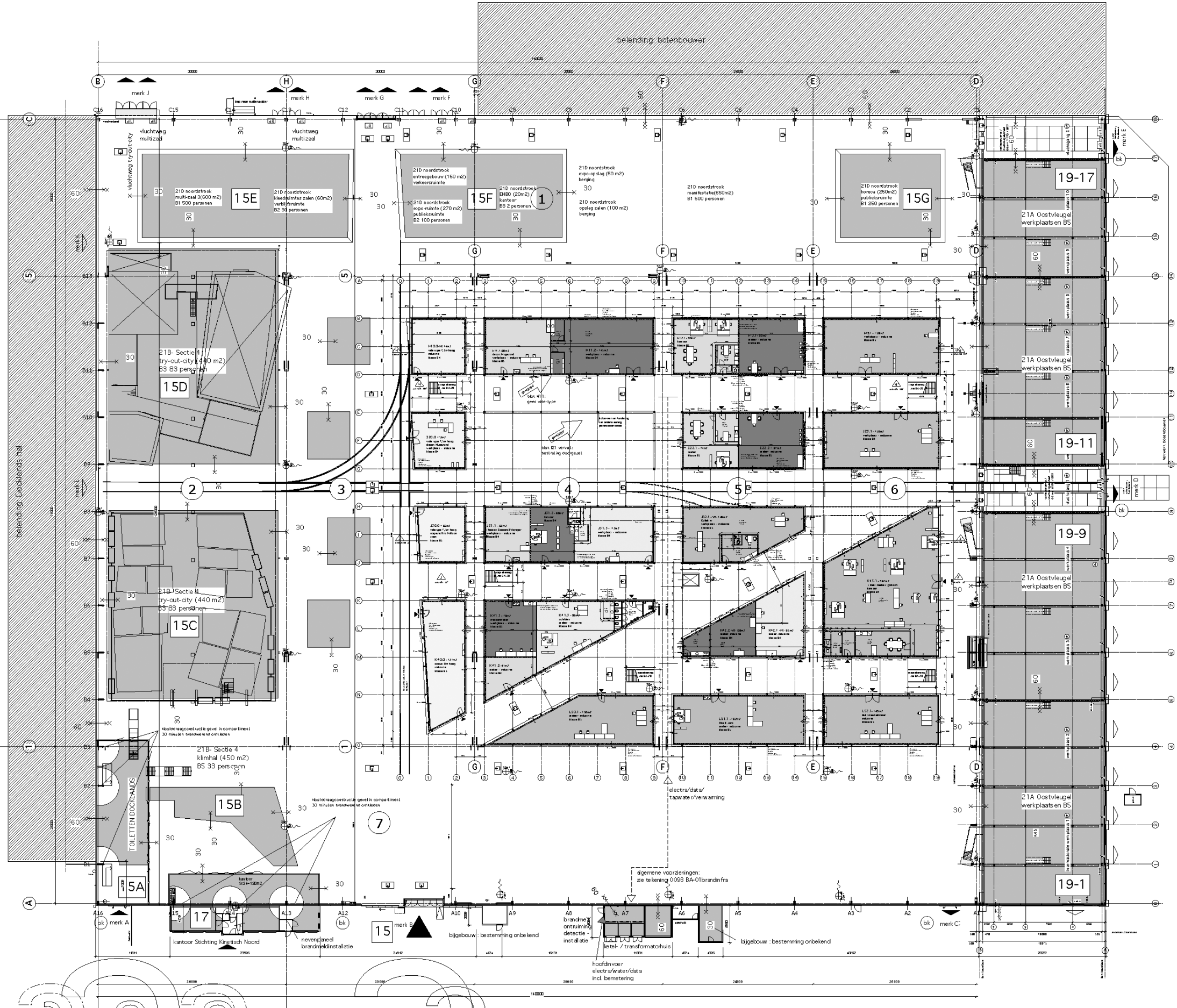
Ground floor / Planta
