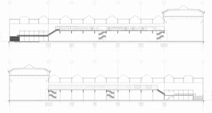
Facade / Fachadas
